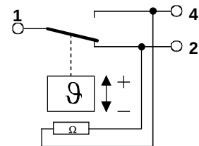
Bellows heater
