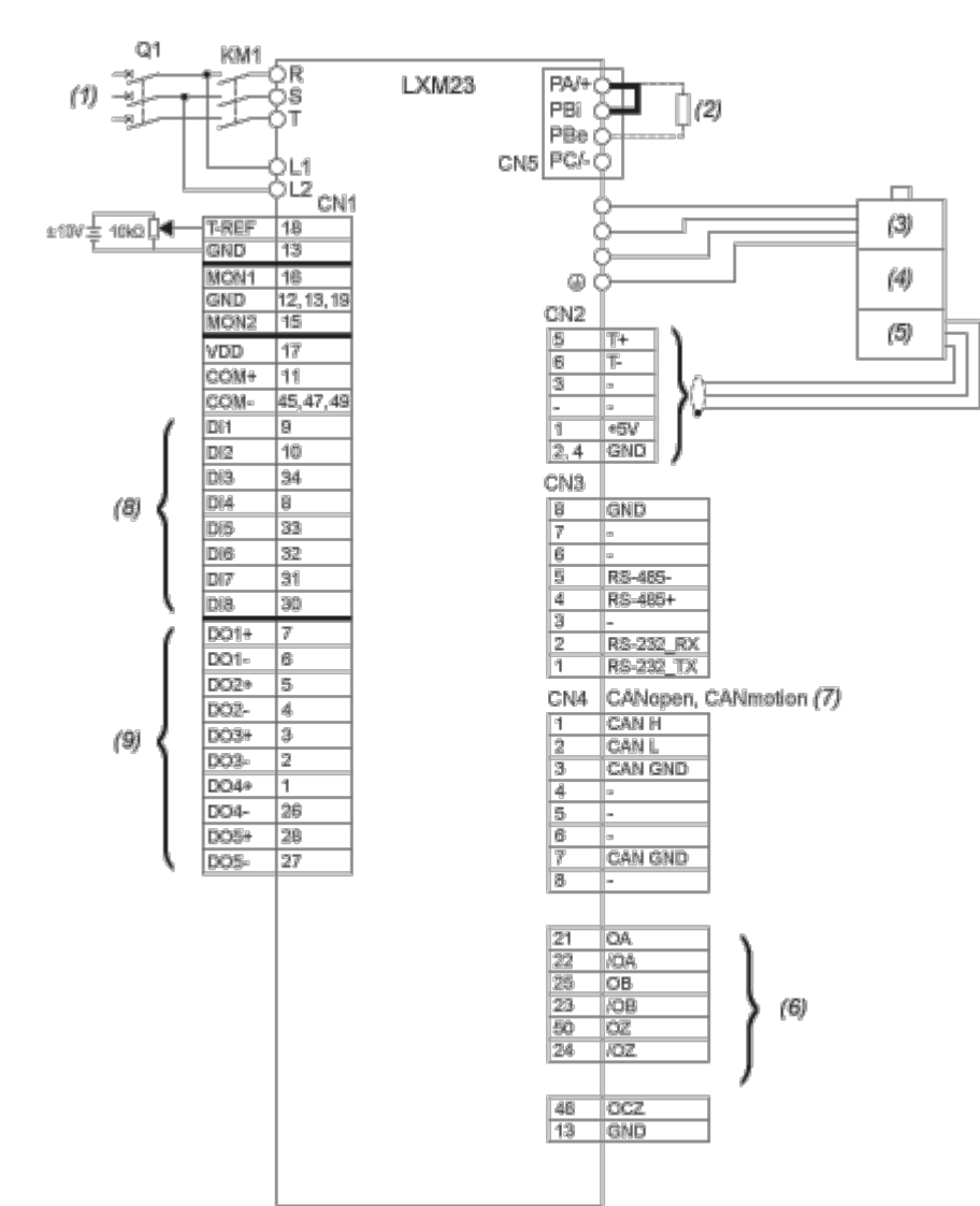
Position Control Mode Wiring Diagram (Build-In Motion Sequence)
