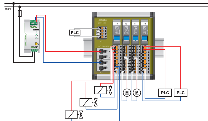
Application drawing
